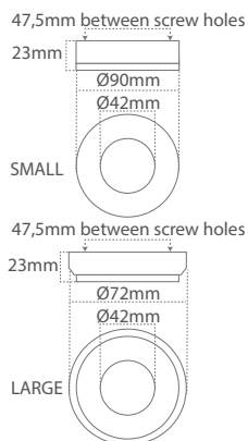
MAJA-SURFACE-SMALL Stainless steel (SS) MAJA-SURFACE-LARGE Stainless steel (SS)
