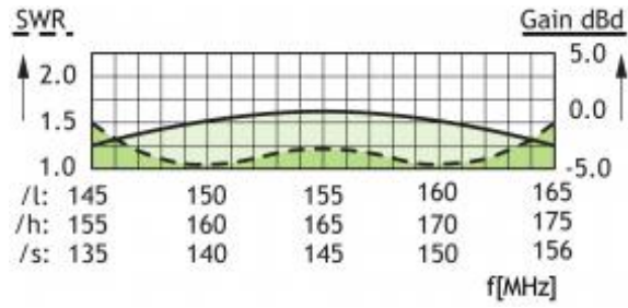
TYPICAL GAIN AND VSWR CURVE
